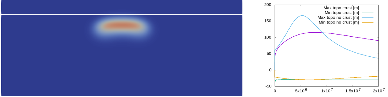
Figure 26: Adding a viscous crust to a model with surface topography. The thermal anomaly spreads horizontally as it collides with the highly viscous crust (left, white solid line). The addition of a crustal layer both dampens and delays the appearance of the topographic maximum and minimum (right).
