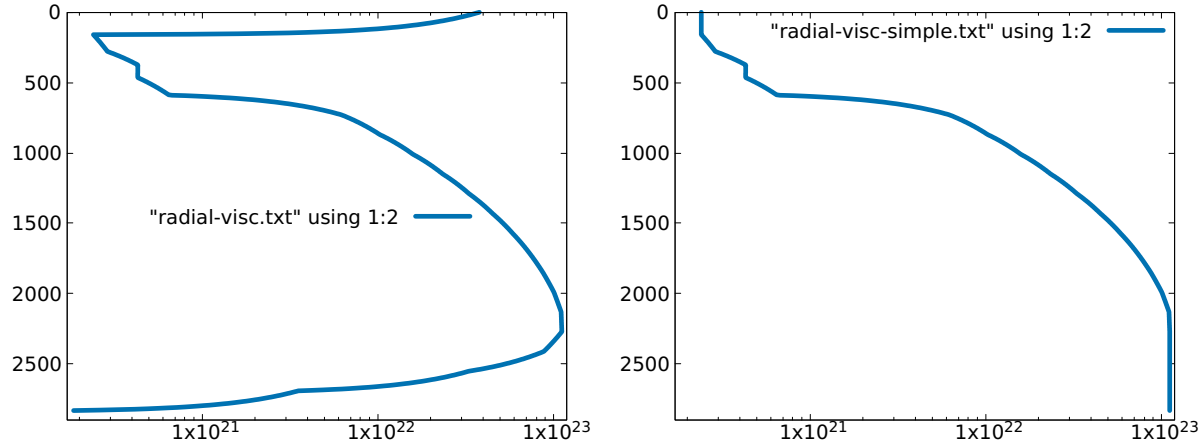
Figure 60: Left: Viscosity profile based on the original [106] formulation, intended for use with a temperature-dependence of viscosity based on the laterally averaged temperature. Right: Modified viscosity profile without boundary layers, intended for use with a temperature-dependence of viscosity based on an adiabatic temperature profile.
