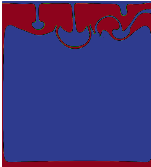
Figure 91: The results of two computations of the van Keken problem made with the VOF interface tracking algorithm overlaid upon each other at t_{end} = 2000 . This visualization shows the reconstructed boundary between the two materials at the final time t_{end} as computed on a uniform grid with 7 and 8 levels of refinement. The boundaries between the materials are displayed as contours of the fields \tilde{\psi}^7(t_{end}) (black) and \tilde{\psi}^8(t_{end}) (bright green), which are generated by the visualization postprocessor. The contours for the reconstructed material boundaries are superimposed on a color gradient visualization of the material composition for the computation with 8 levels of refinement in order to make the regions with each fluid type more evident. Compare with the fourth image on the right in Figure 81.
