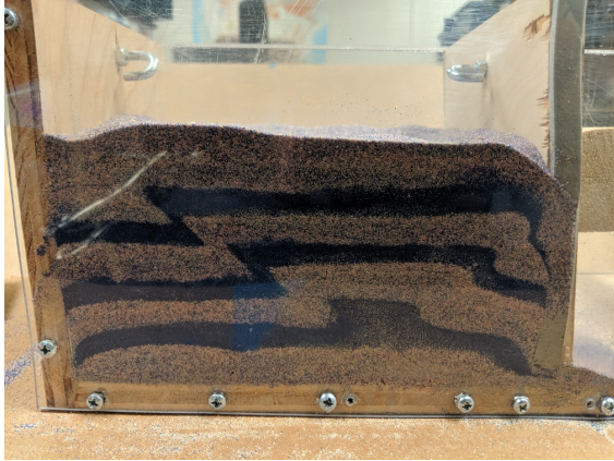
Figure 140: Examples of deformation patterns of “sand box” experiments in which alternating layers of differently-colored sand undergo deformation. Pictures courtesy of the lab of Dennis Harry at Colorado State University.
