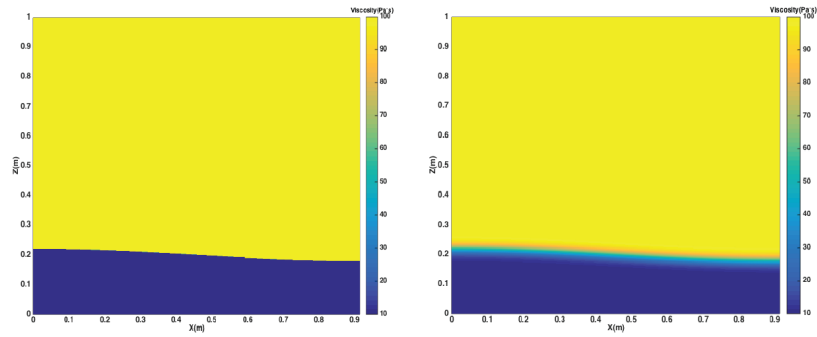
Figure 87: Van Keken benchmark using different-viscosity layers. The left image is the discontinuous case, while right is the smooth. Both are shown at t = 0 .
