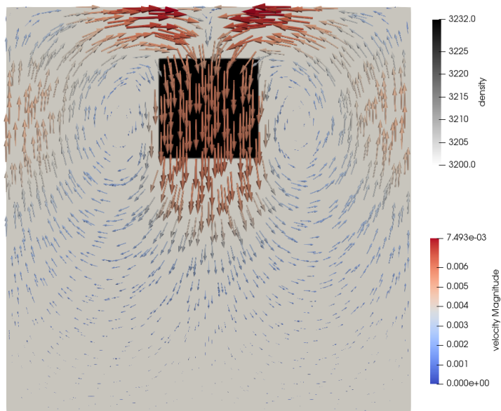
Figure 99: Density field with velocity arrows for \eta_2 = 10^{27} Pa s and \delta\rho = 32 kg m ^{-3}
