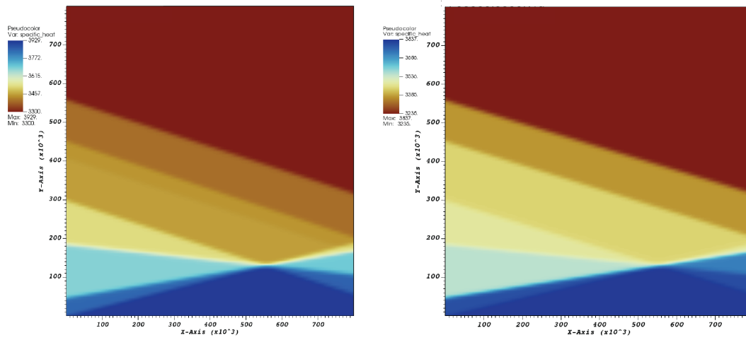
Figure 40: Visualization of phase diagrams: The field of heat capacity showing values of reference densities for pyrolitic and harzburgitic phases.
