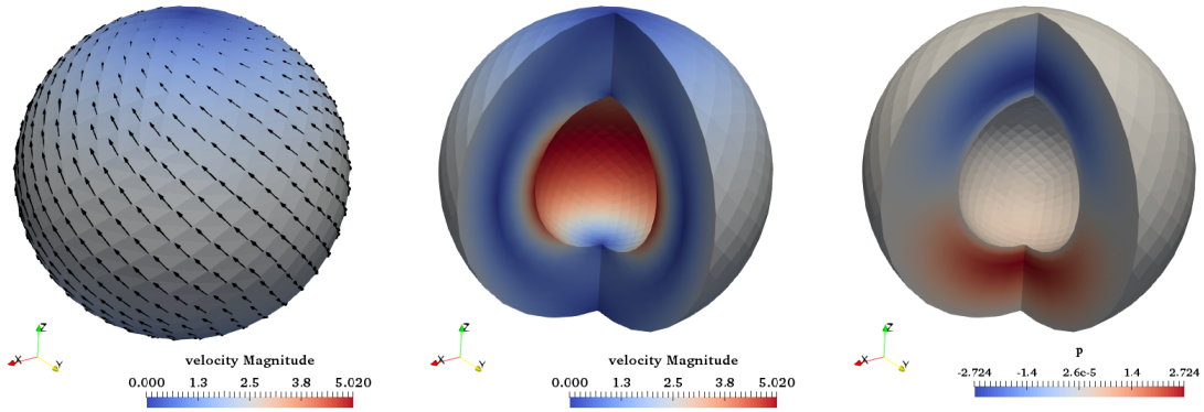
Figure 109: Velocity and pressure fields for the hollow sphere benchmark.
