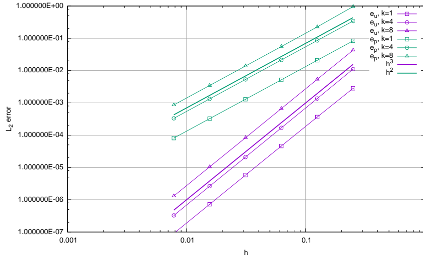
Figure 112: Velocity and pressure errors in the L_2 -norm as a function of the mesh size for the 2D annulus benchmark.
