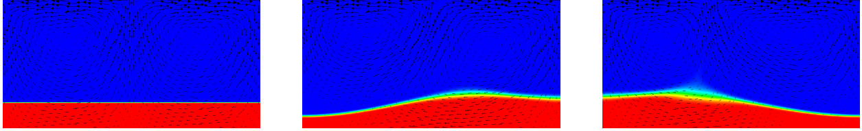
Figure 20: Active compositional fields: Compositional field 1 at the time t = 0, 10, 20 . Compared to the results shown in Fig. 17 it is clear that the heavy material stays at the bottom of the domain now. The effect of the density on the velocity field is also clearly visible by noting that at all three times the spreading center at the top boundary is in exactly the same position; this would result in exactly the same velocity field if the density and temperature were constant.
