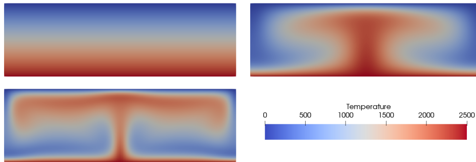
Figure 145: Onset of convection model with different Rayleigh numbers. Background colors show temperature.
