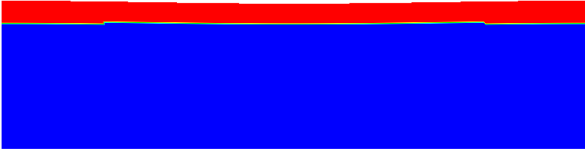
Figure 122: Setup for the topography relaxation benchmark. The box is 2800 km wide and 700 km high, with a 100 km lid on top. The lid has a viscosity of 10^{23} Pa s, while the mantle has a viscosity of 10^{21} Pa s. The sides are free slip, the bottom is no slip, and the top is a free surface. Both the lid and the mantle have a density of 3300 \text{ kg/m}^3 , and gravity is 10 \text{ m/s}^2 . There is a 7 km sinusoidal initial topography on the free surface.
