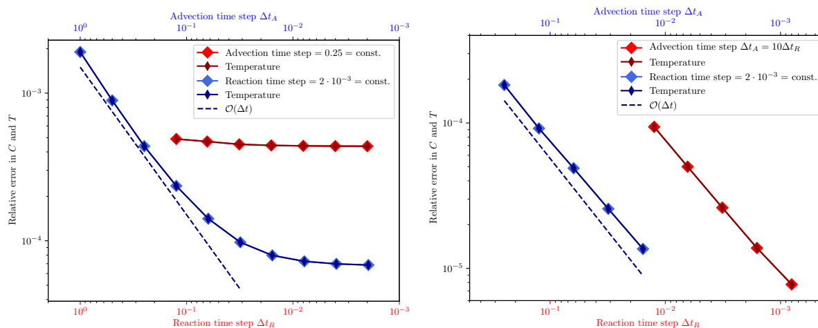
Figure 129: Error for both compositional field and temperature compared to the analytical solution, varying the time steps of advection (blue data points and top/blue x axis) and reactions (red data points and bottom/red x axis), while keeping the other one constant, respectively.
