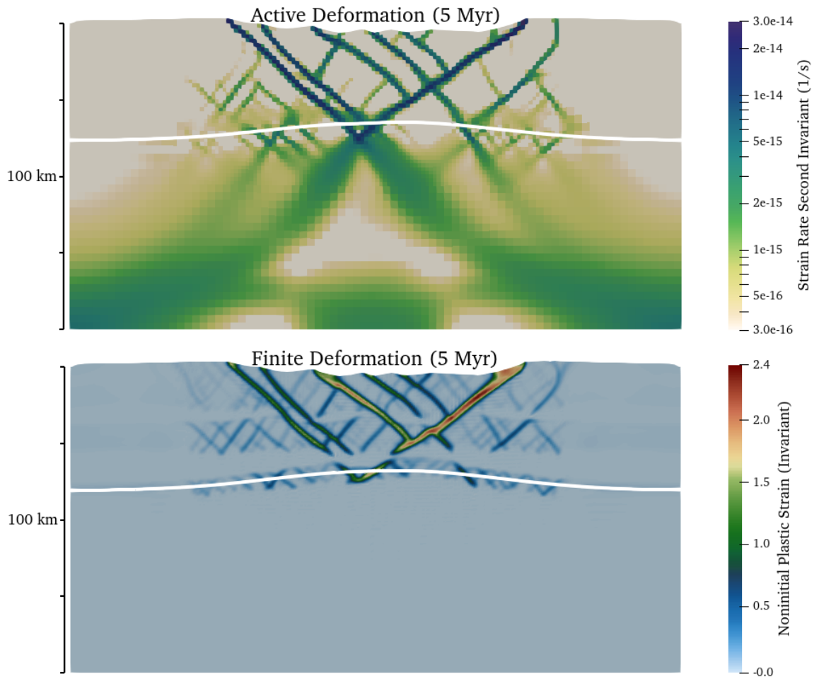
Figure 68: Active (strain rate second invariant in units of s^{-1} ) and finite (plastic) deformation after 5 \times 10^6 years of extension. The white line marks the (893 K) isotherm (initial Moho temperature).
