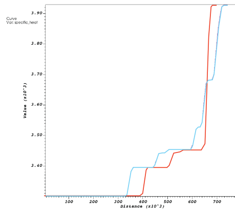
Figure 41: Visualization of phase diagrams: Profiles of pyrolitic density at T = 1173\text{ K} (red) and 1673\text{ K} (blue).
