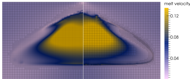
Figure 75: Mesh after a time of 3.6 million years for a model using the composition threshold refinement strategy (left) and the compaction length refinement strategy (right). Background colors indicate the melt velocity. Its sharp gradients at the interface between regions with and without melt can only be resolved using the compaction length refinement strategy.
