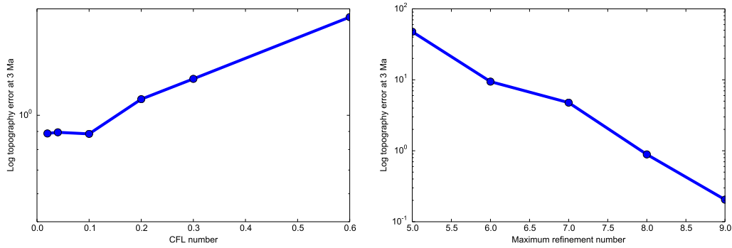
Figure 126: Convergence for case two. Left: Logarithm of the error with decreasing CFL number. As the CFL number decreases, the error gets smaller. However, once it reaches a value of \sim 0.1 , there stops being much improvement in accuracy. Right: Logarithm of the error with increasing maximum mesh resolution. As the resolution increases, so does the accuracy.
