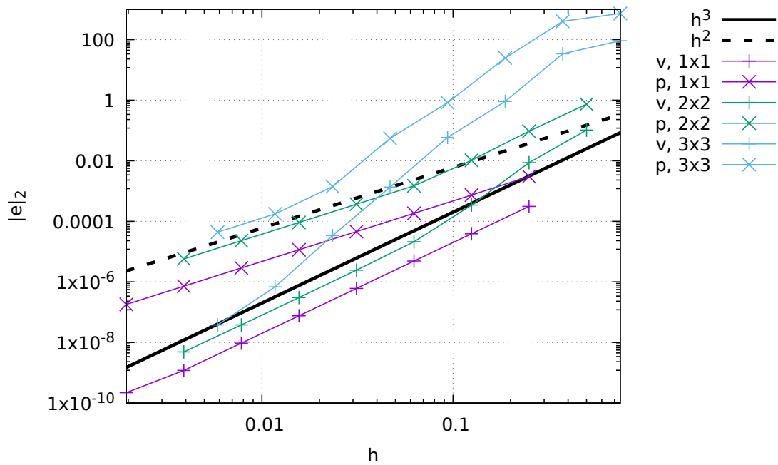
Figure 117: Viscosity grooves benchmark: Velocity and pressure error convergence as a function of the mesh size h for 3 domain sizes.
