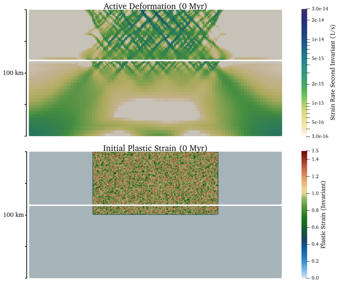
Figure 67: Initial active deformation field (strain rate second invariant in units of \text{s}^{-1} ) and distribution of plastic strain. The white line marks the (893 K) isotherm (initial Moho temperature).
