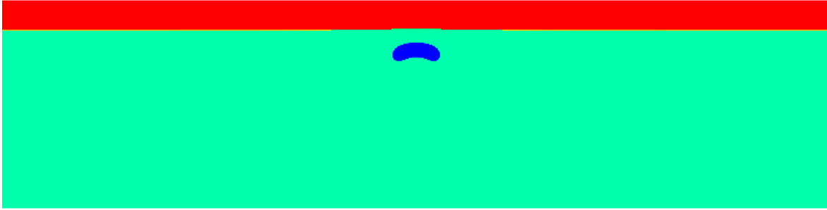
Figure 124: Setup for the dynamic topography benchmark. Again, the domain is 2800 km wide and 700 km high. A 100 km thick lid with viscosity 10^{23} overlies a mantle with viscosity 10^{21} . Both the lid and the mantle have a density of 3300 \text{ kg/m}^3 . A blob with diameter 100 km lies 300 km from the bottom of the domain. The blob has a density of 3200 \text{ kg/m}^3 and a viscosity of 10^{20} \text{ Pa s} .
