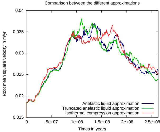
Figure 59: Comparison between the anelastic liquid approximation, the truncated anelastic liquid approximation and the isothermal compression approximation, showing the evolution of the root mean square velocity.
