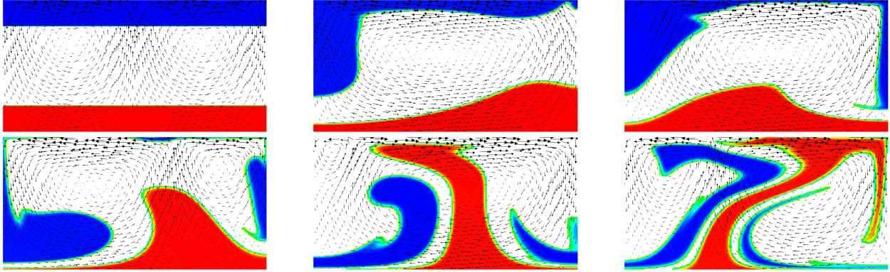
Figure 17: Passive compositional fields : The figures show, at different times in the simulation, the velocity field along with those locations where the first compositional field is larger than 0.5 (in red, indicating the locations where material from the bottom of the domain has gone) as well as where the second compositional field is larger than 0.5 (in blue, indicating material from the top of the domain). The results were obtained with two more global refinement steps compared to the cookbooks/composition_passive/composition_passive.prm input file.
