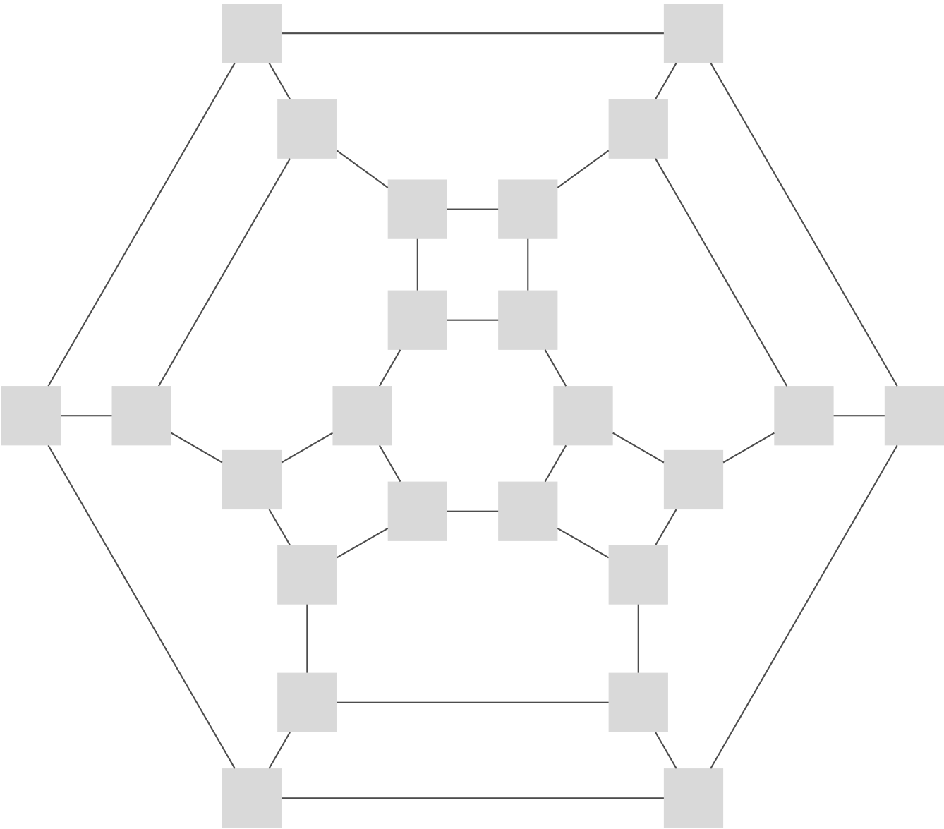
#3(a): Cayley graph for the second mystery group, labeled with square tiles.
