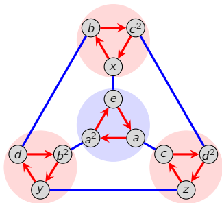
Cluster the left cosets of H = \langle(123)\rangle .
