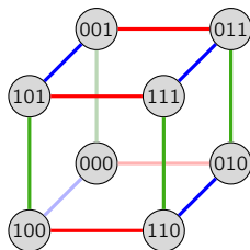
\mathbb{Z}_2 \times \mathbb{Z}_2 \times \mathbb{Z}_2 \cong \text{Light}_3
