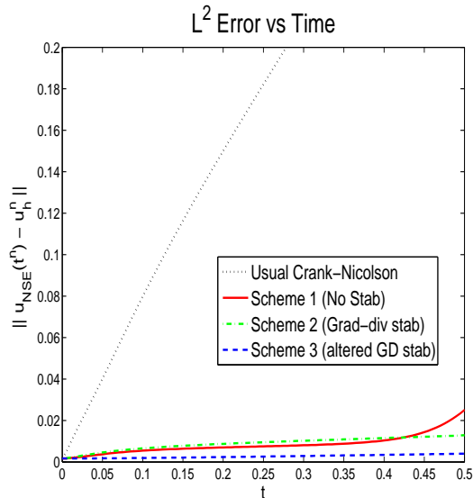
Figure 2: The plot above shows L_2 error of the velocity vs time for the four schemes of Test 2. We see in the plot that the stabilizations add accuracy to the enhanced-physics scheme, and that the alternate grad-div stabilization gives slightly better results than the usual grad-div stabilization. It can also be seen that the enhanced-physics scheme is far more accurate in this metric than the usual CCN scheme.
