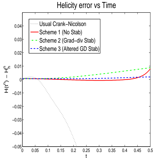
Figure 3: The plot above shows helicity error vs time for the four schemes of Test 2. We see in the plot that helicity is far more accurate in the enhanced-physics scheme, and even better with stabilizations, than the usual CCN scheme.
