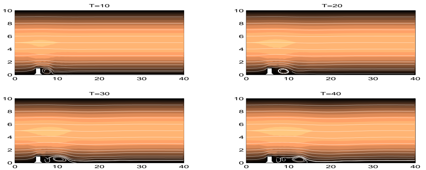
Figure 4.10: NSE + NTR0 at \nu = 1/600 , \delta = 1.5 and level 1 grid
