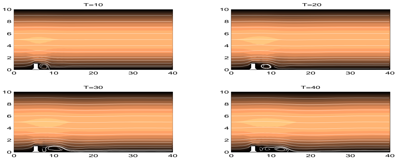
Figure 4.9: NSE + TR1 at \nu = 1/600 , \delta = 1.5 and level 1 grid
