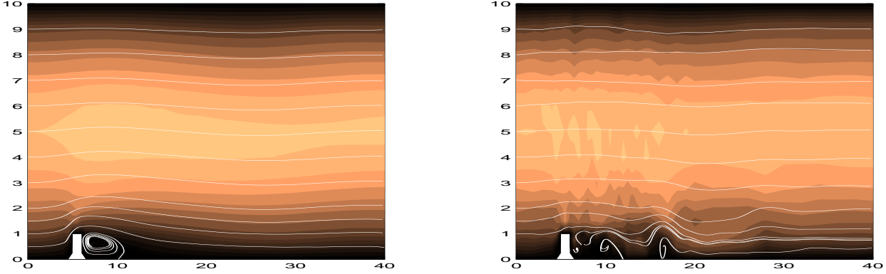
Figure 4.11: NSE+SM (left) and NSE+NTR0 (right) at \nu = 1/600 , \delta = 3.0 , level 0 grid
