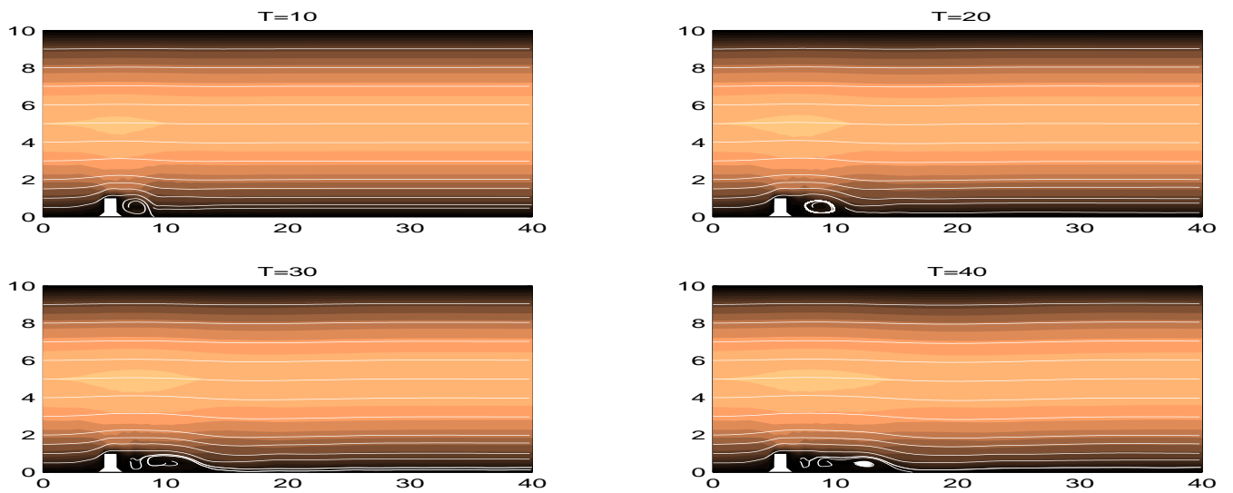
Figure 4.8: NSE + TR0 at \nu = 1/600 , \delta = 1.5 and level 1 grid
